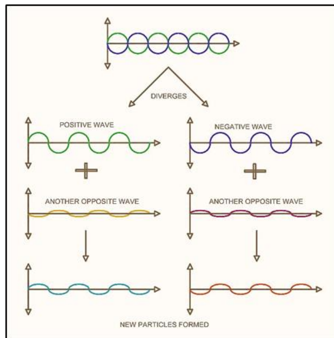
fig. 7: formation of waves and then particles.
