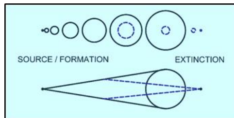
fig. 4: diagram of simplified model of every naturally occurring substance.
