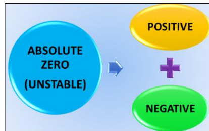
fig. 6: evolution from nothing.
