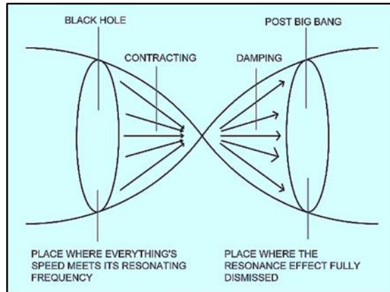
fig. 3: diagram of process in between black hole and post big bang.
