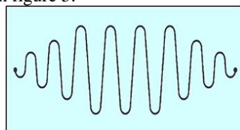
fig. 5: diagram of wave.
