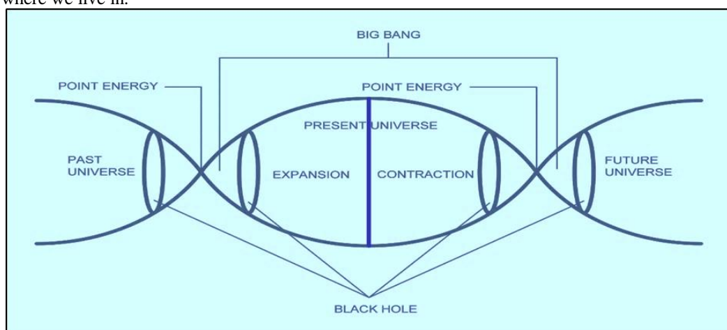
fig. 2: diagram of the creation, destruction and recreation of universe.
