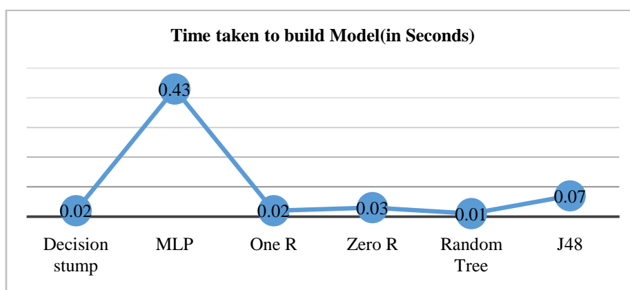
Figure 3. Time taken by the classifiers
