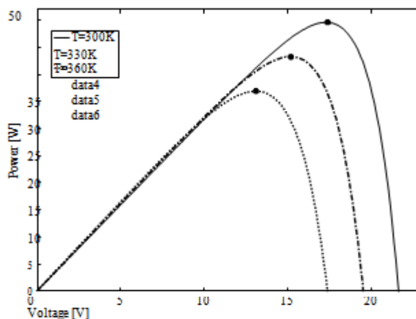
Fig. 4. V-P panel characteristics for three different temperature levels. Each point represents the MPP of related curve.
